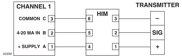
Figure 6—Three-Wire Transmitter / Detector with HART Interface Module — Non-Isolated 4 to 20 mA Current Output (Sourcing)
